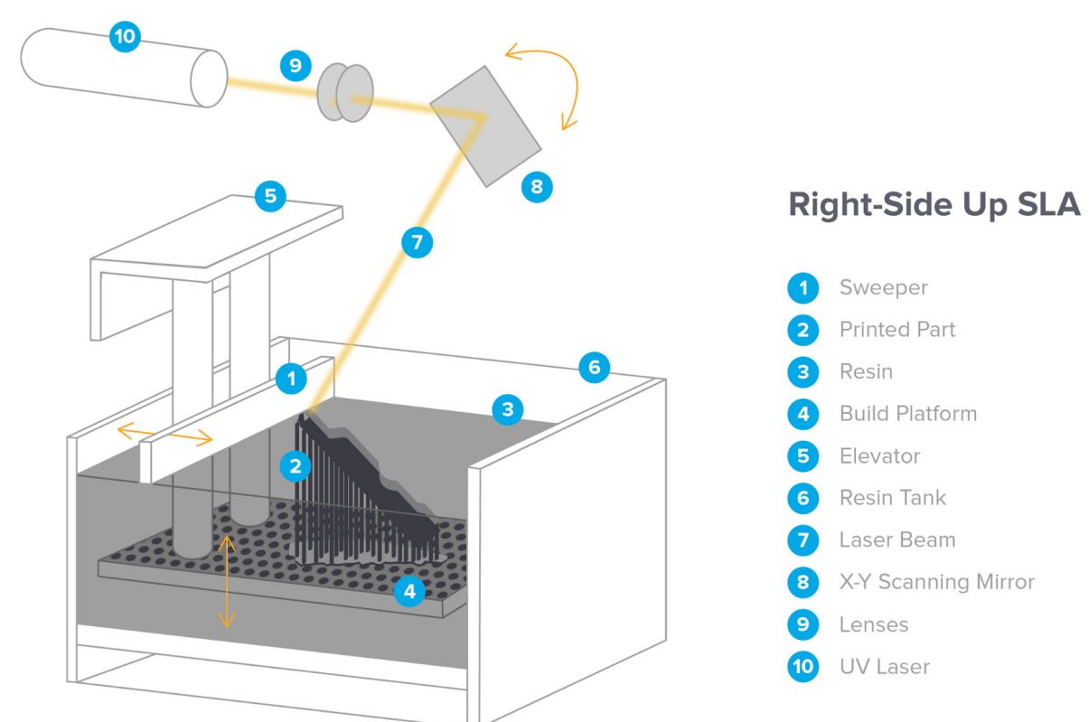
Schematic of the right-side up SLA systems.
