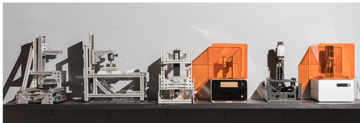
Prototypes of the Form 1, the first desktop SLA 3D printer
