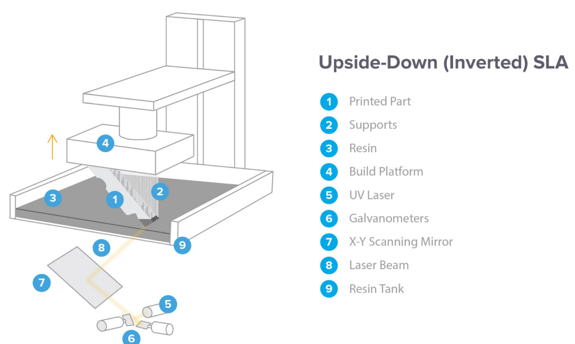
Schematic of the upside-down (inverted) SLA systems
