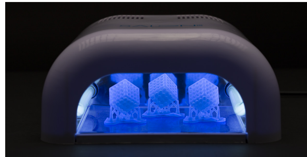
SLA prints in a UV-curing station. UV post-curing finalizes the polymerization process and stabilizes the mechanical properties.
